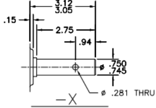
-X SEE DWG. M164-1X USE #8648 OIL SEAL
