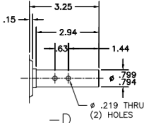
-D SEE DWG. M164-1D USE #8648 OIL SEAL
