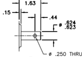
-R SEE DWG. M164-1R USE #6372 OIL SEAL
