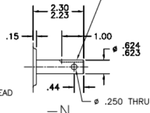
-N SEE DWG. M164-1N USE #6372 OIL SEAL
