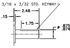
-7K SEE DWG. M164-1-7K USE #8648 OIL SEAL
