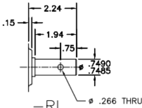
-RL SEE DWG. M164-1RL USE #8648 OIL SEAL
