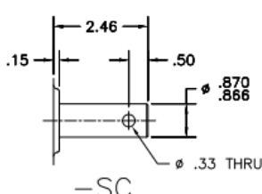
-SC SEE DWG. M164-1SC USE #8648 OIL SEAL
