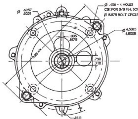
Rear View (Input end) Mounting Dimensions for NEMA 56C Motor
