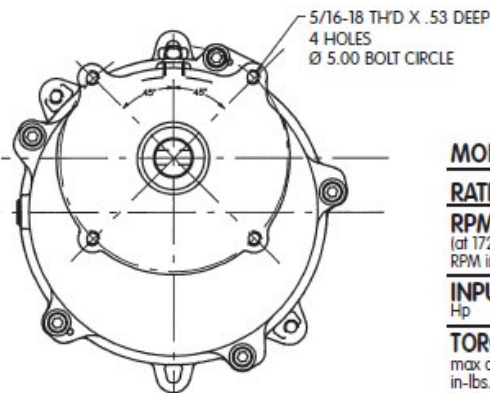
Front View (Output end)
